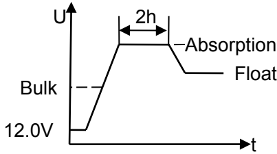
Figure 2-2: Three-stage Charge
