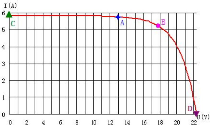
Figure 2-4: Voltage-Current Curve
