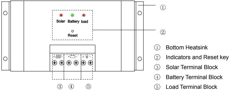
Figure 2-1: Controller Structure Diagram
