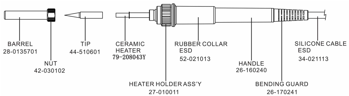
Fig. 1 Soldering iron assembly
